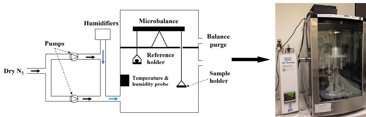
Fig. 2. Schematic illustration of the gravimetric analyzer for the measurement of water
