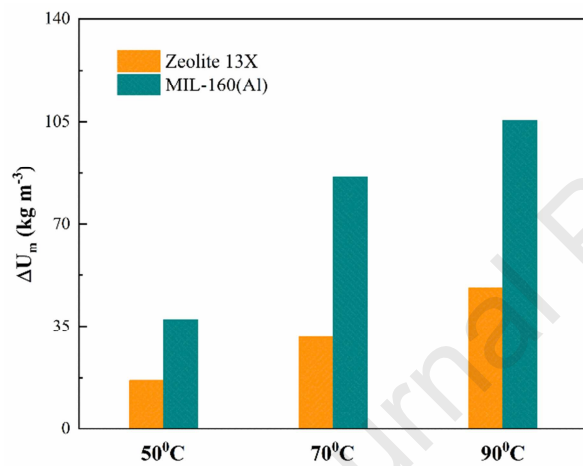
Fig. 12 The effect of regeneration temperature on the net cyclic capacity.
