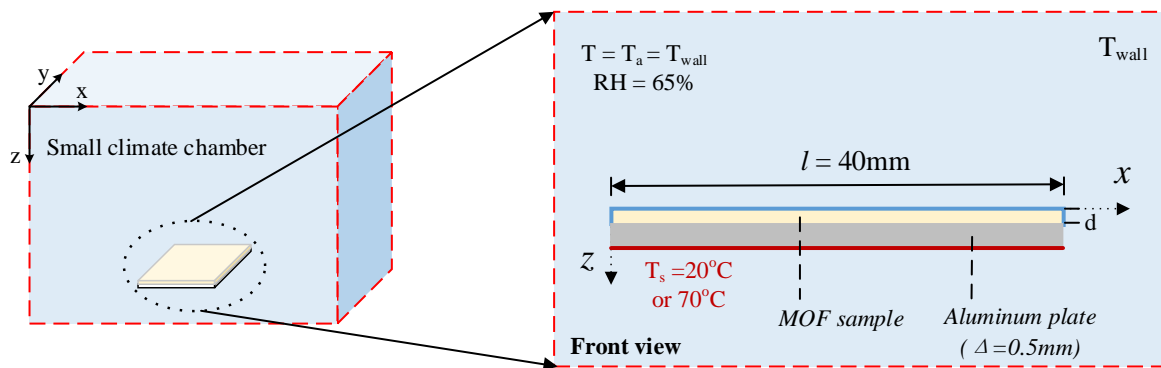
Fig. 4. The schematic of the simulation model
