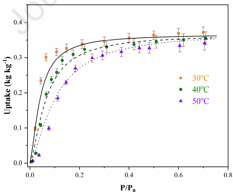
Fig. 5. Sorption isotherms of MIL-160(Al) under different temperature conditions. Here,
