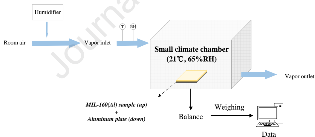
Fig.3 The setup of sorption performance tests.
