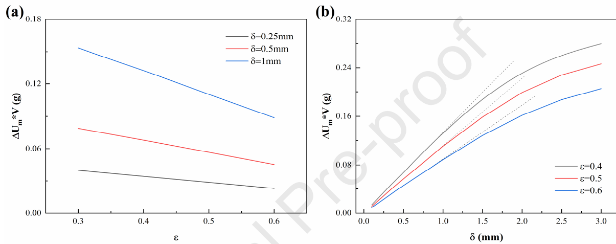
Fig. 11 Variation of the net cyclic capacity shown as a function of a) porosity and b) thickness.
