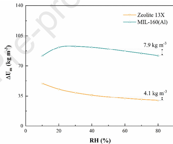
Fig. 13 The effect of the surrounding vapor pressure on the net cyclic capacity ( T_{\text{reg}}=70^\circ\text{C} ).
