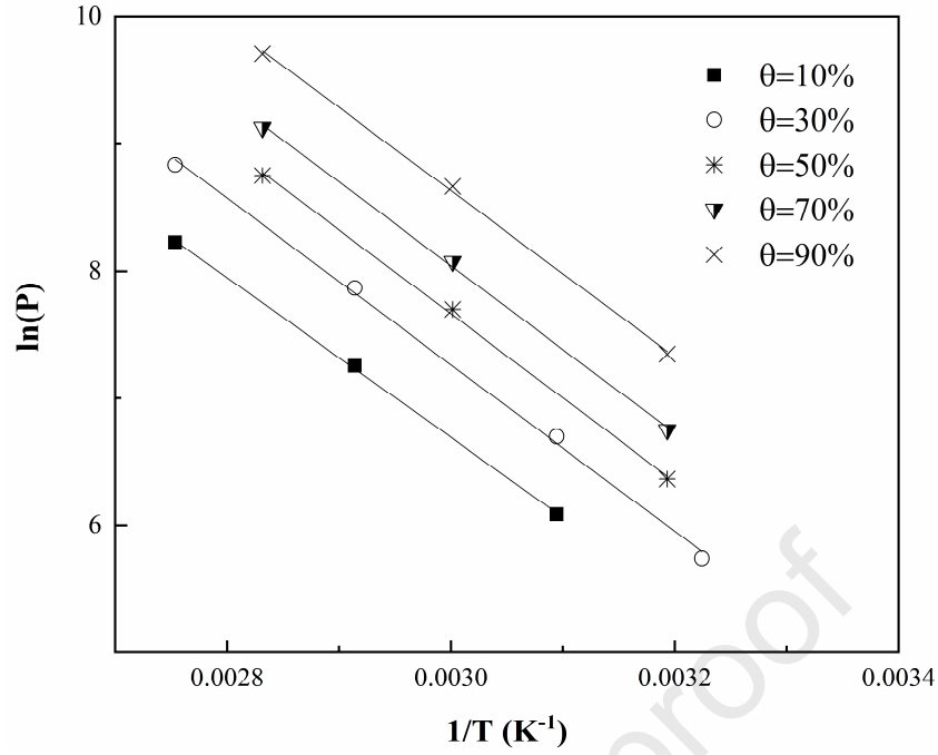
Fig. 6. Isotheric heat of water vapor adsorption on MIL-160(Al) for different water uptake fractions.
