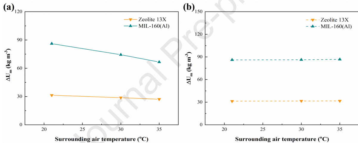
Fig. 14 The effect of different surrounding air temperatures on the net cyclic capacity ( T_{\text{reg}}=70 ). a) RH=65\% ; b) \rho_0=0.0118 \text{ kg m}^{-3} .
